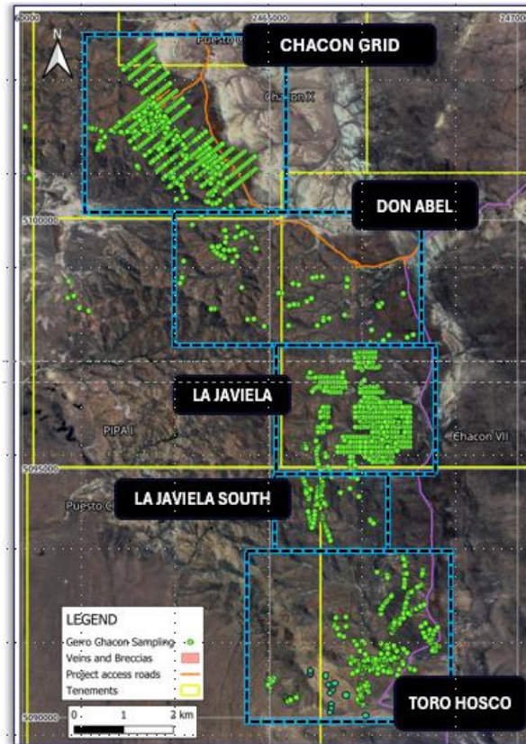
Figure 1 Rock Chip and soil geochemical samples at Chacón Projects
